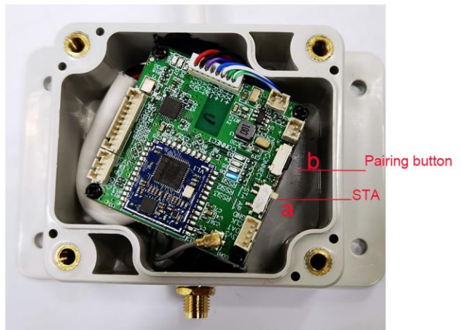
STA sender for IP equipment (IP camera)
