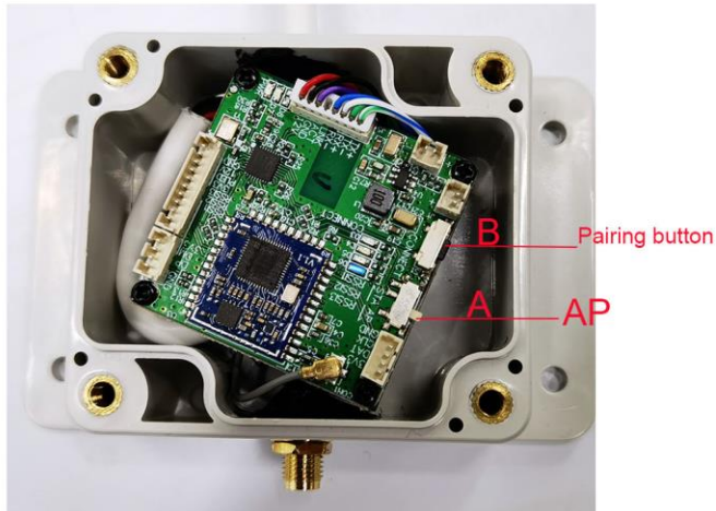
AP Receiver for Switch/router
